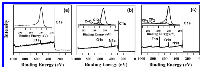
Figure 3. XPS spectra of (a) the pristine aligned carbon nanotube film, (b) the AZT-grafted side, and (c) the perfluorooctyl chain-grafted side of an aligned A-CNT-F film, along with the corresponding high-resolution C 1s spectra.
